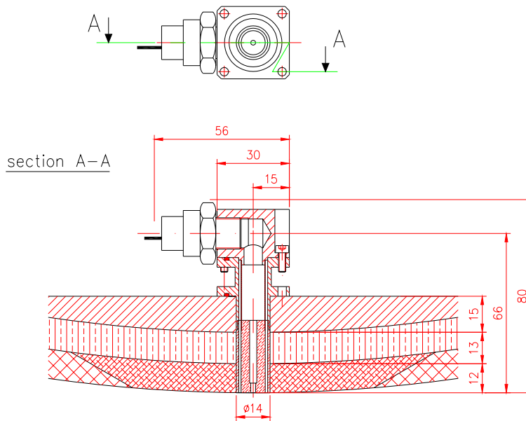
Fig.17 Installation drawing of RAFLEX III in stagnation point of IRDT
