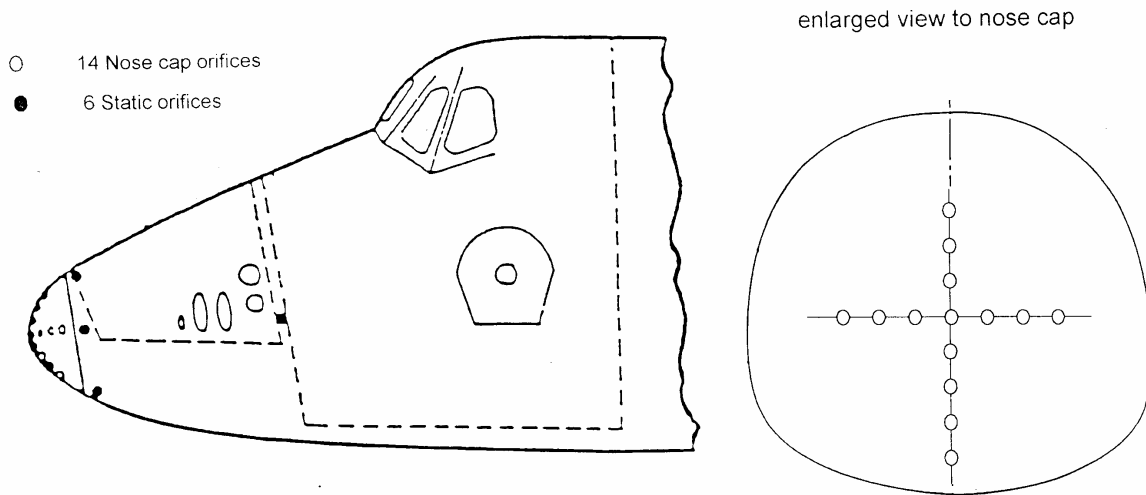
Fig. 10 Principle of Shuttle Entry Air Data system SEADS
